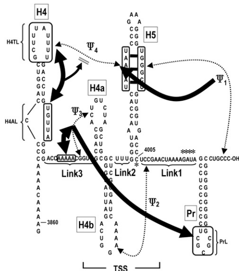
FIGURE 8. Interactions between different elements in the 3' UTR of TCV. Thick arrows reflect interactions that are disrupted when elements are mutated. For example, mutation in \Psi_3 affect the structure of the adjacent adenylates (and vice versa, indicated by double arrowheads) and the structure of PrL (single arrowhead, since the reverse is not known); mutations in \Psi_1 affect the structure of non-Watson-Crick interactions across the H5 LSL; however, mutations in the 5' side of the H5 LSL do not abrogate \Psi_1 . Asterisks indicate residues in "hinge" locations that are sterically affected by disruption of some of the interactions (see text for more details), or some differences following the RdRp-mediated conformational shift.
