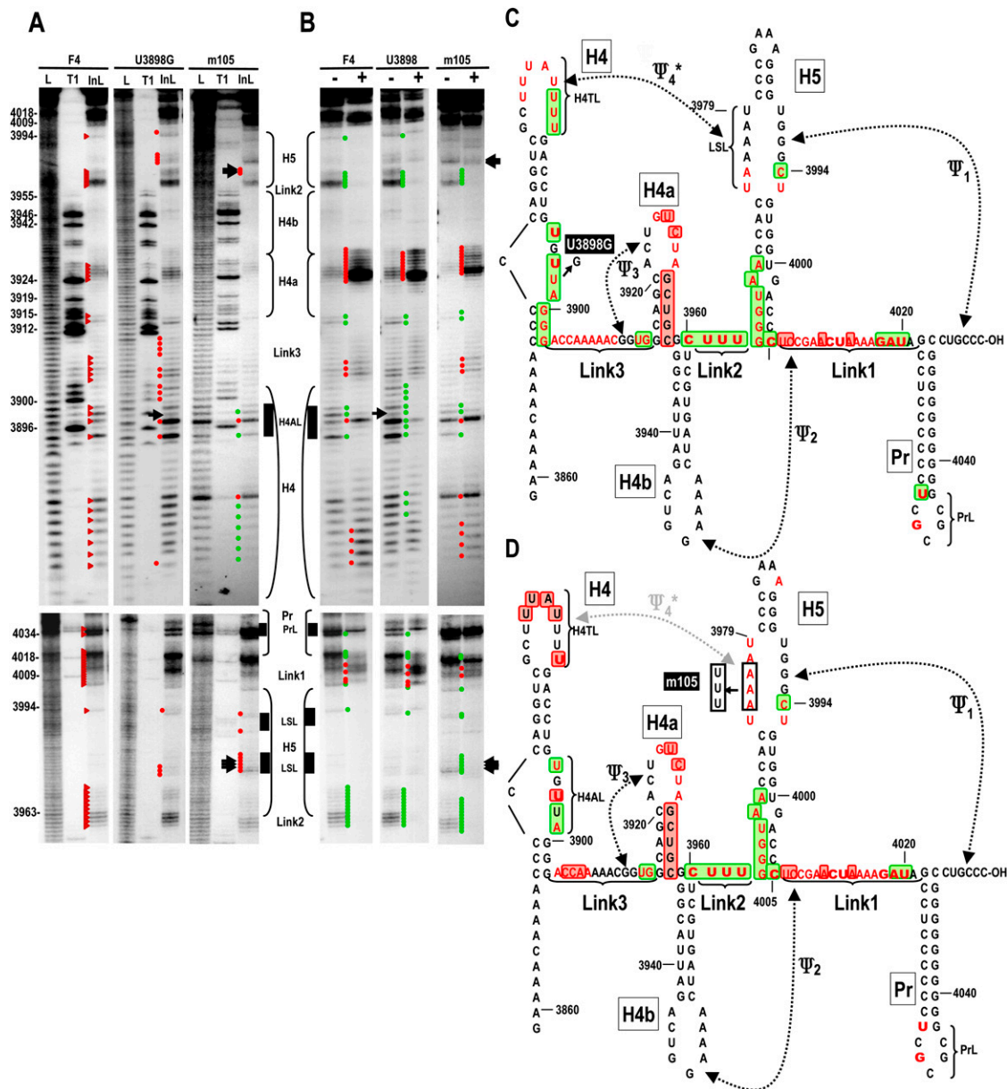
FIGURE 5. Mutations in H4AL or H5 LSL affect the structure of H4AL, H5 LSL, and H4TL. (A) In-line cleavage of transcripts containing mutations in H4AL (U3898G) or H5 LSL (m105). Location of the mutations are shown in C and D. See the legend to Figure 2A for further details. (B) Structural alterations in the presence of MBP-RdRp. See the legend to Figure 2B for further details. (C) Structural alterations in F4 due to U3898G, and (D) m105 in the presence and absence of MBP-RdRp. See the legend to Fig. 2C for details.
