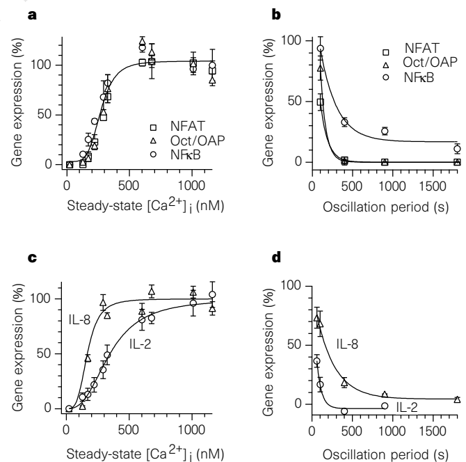
Figure 3 Effects of [\text{Ca}^{2+}]_i and oscillation frequency on NF-AT-, Oct/OAP-, NF- \kappa B-, IL-2- and IL-8-luciferase reporter genes. a , Steady-state \text{Ca}^{2+} sensitivities of NF-AT, Oct/OAP and NF- \kappa B. A plot of the Hill equation is superimposed, with a Hill coefficient ( n_H ) of 4.7 and a K_d of 270 nM. b , Oscillation frequency dependences of NF-AT (□), Oct/OAP (Δ) or NF- \kappa B (○) reporter genes. c , Steady-state \text{Ca}^{2+} sensitivities of IL-2 (○) and IL-8 (Δ) reporter genes. Fits to the Hill equation are superimposed (for IL-2, n_H = 2.7 and K_d = 346 nM; for IL-8, n_H = 3.6 and K_d = 166 nM). d , Frequency dependences of IL-2 (○) and IL-8 (Δ) reporter genes. Error bars represent s.e.m. of triplicate measurements in 3–5 experiments; where they are not visible they are smaller than the symbols. All experiments were done in the presence of 50 nM PdBu.
