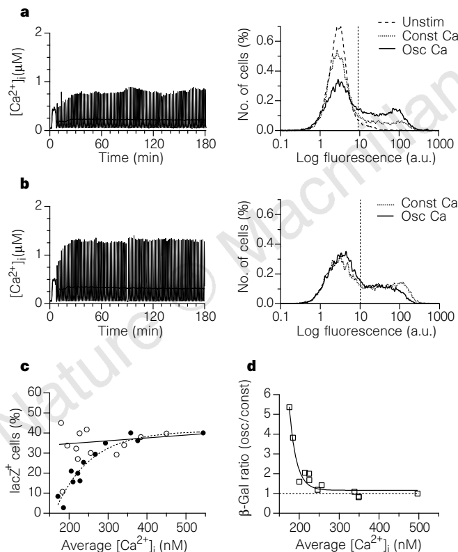
Figure 2 [\text{Ca}^{2+}]_i oscillations enhance the calcium sensitivity of NF-AT-dependent transcription at low levels of stimulation. a , NF-AT-dependent lacZ expression in cells stimulated with a low level of [\text{Ca}^{2+}]_i . Left, superimposed [\text{Ca}^{2+}]_i recordings from two cell populations (200–300 cells each) stimulated for 3 h with oscillating [\text{Ca}^{2+}]_i (227 nM average) or constant [\text{Ca}^{2+}]_i (225 nM average). Right, flow cytometry analysis of \beta -gal activity in the same experiments show that oscillating [\text{Ca}^{2+}]_i activates 39% of the cells while constant [\text{Ca}^{2+}]_i activates only 19%. The vertical gate excludes 97% of the unstimulated cells. b , NF-AT-dependent expression at a high level of [\text{Ca}^{2+}]_i . Left, stimulation with oscillating [\text{Ca}^{2+}]_i (340 nM average) or constant [\text{Ca}^{2+}]_i (359 nM average). Right, oscillating and constant [\text{Ca}^{2+}]_i activate 33 and 39% of the cells, respectively. c , Percentage of lacZ + cells induced by various concentrations of oscillating (○) or constant (●) [\text{Ca}^{2+}]_i . d , Ratio of the number of \beta -gal + cells activated by oscillating as compared with constant [\text{Ca}^{2+}]_i , as a function of average [\text{Ca}^{2+}]_i , calculated from the data in c . All experiments were done in the presence of 50 nM PdBu.
