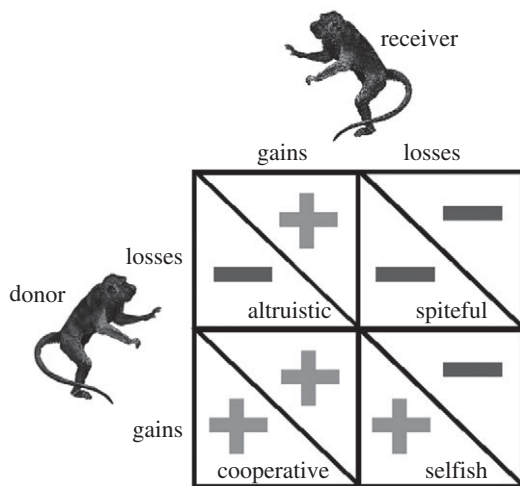
Figure 1. A social matrix of interactions based on gains (plus) and losses (minus) to the donor and recipient.
